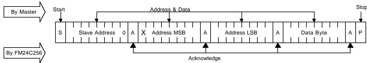
Figure 5 Byte Write
