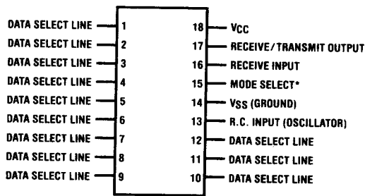
18-Pin DIP — Top View
