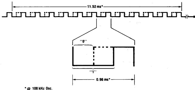
Figure 1. Output Waveform
