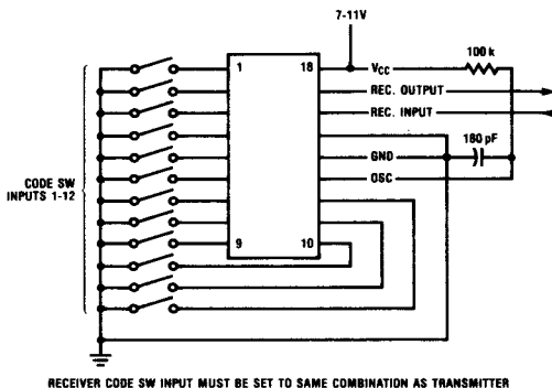
Figure 2. Pin Connections for Receiver Mode
