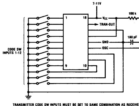
Figure 3. Pin Connections for Transmitter Mode
