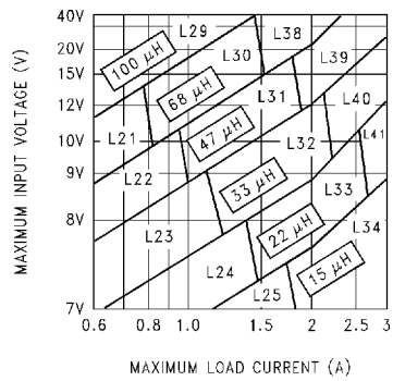
FIGURE 6. LM2596-5.0
