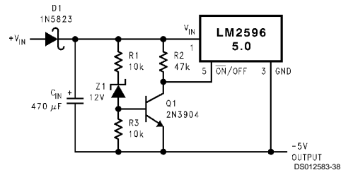
FIGURE 23. Undervoltage Lockout for Inverting Regulator
