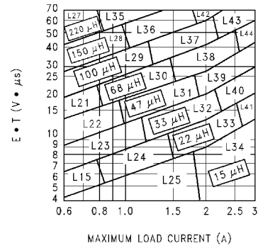
FIGURE 8. LM2596-ADJ
