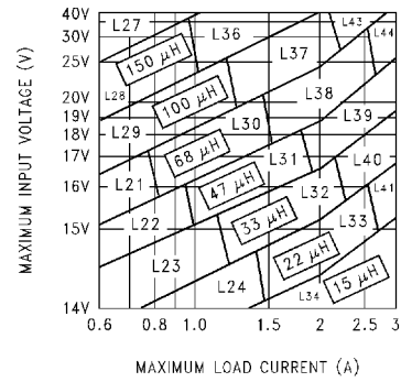
FIGURE 7. LM2596-12
