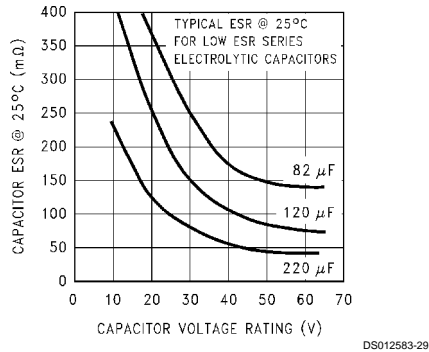
FIGURE 14. Capacitor ESR vs Capacitor Voltage Rating (Typical Low ESR Electrolytic Capacitor)
