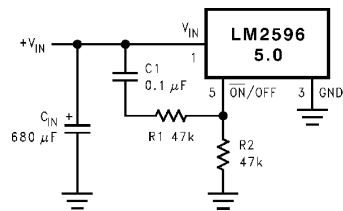
FIGURE 21. Delayed Startup
