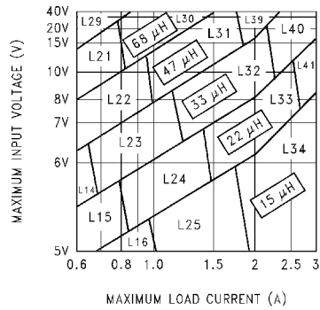
FIGURE 5. LM2596-3.3
