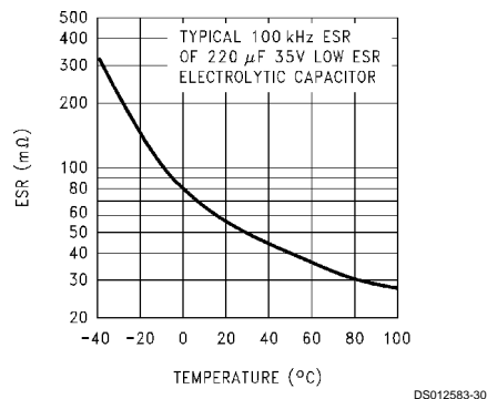
FIGURE 15. Capacitor ESR Change vs Temperature
