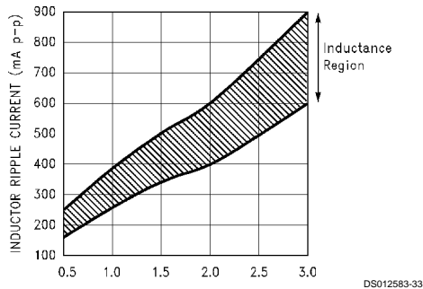
FIGURE 18. Peak-to-Peak Inductor Ripple Current vs Load Current
