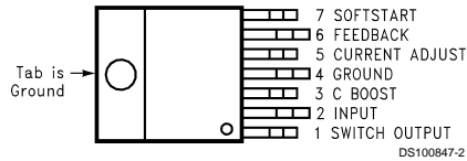
TO-220 Package Top View
