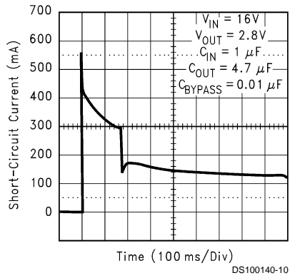
Short-Circuit Current
