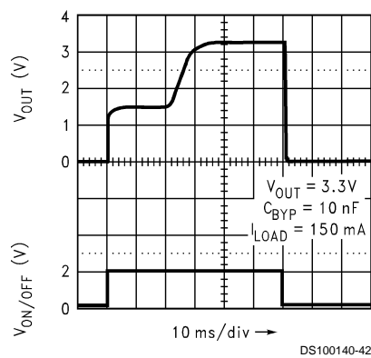
Turn-On Time
