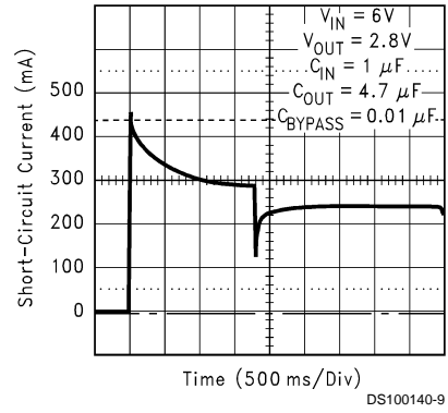
Short-Circuit Current
