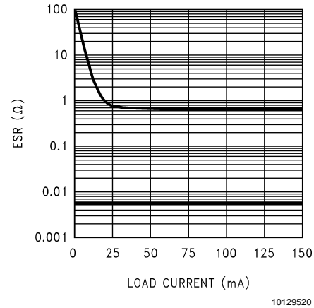
FIGURE 2. LP2985LV 4.7 \mu\text{F} Stable ESR Range
