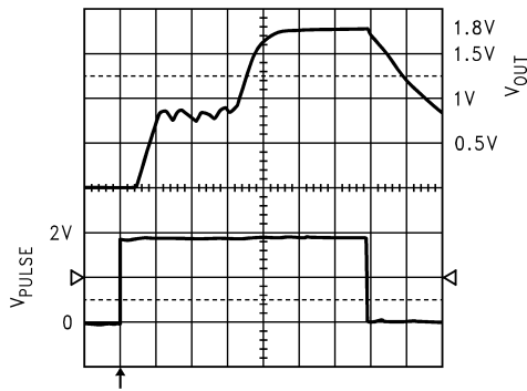
Turn-On Time
