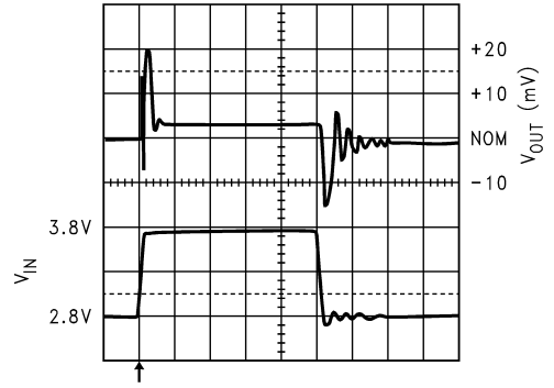
Line Transient
