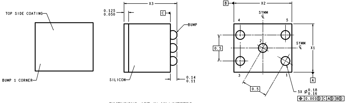
DIMENSIONS ARE IN MILLIMETERS
