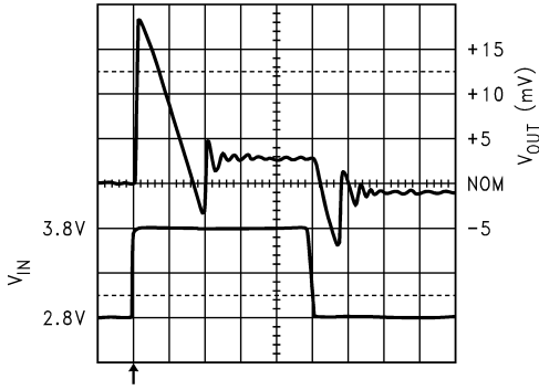
Line Transient
