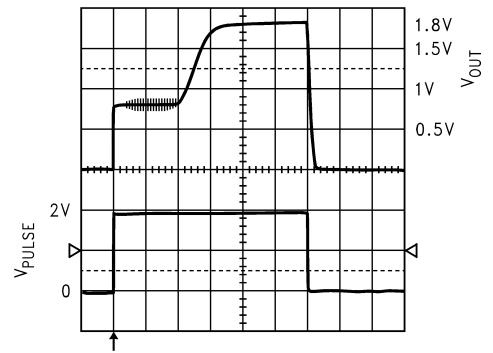
Turn-On Time
